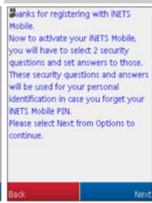
Select Next
